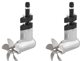
2 x Pod Drive 12 eSSA Total Power: 24 kW
