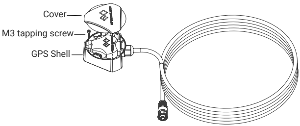
Figure 4.20 GPS External Module Screw Fixing
