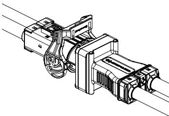
Figure 4.12 High-voltage interlock connector - Installation step 3
