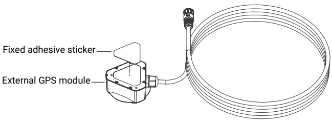
Figure 4.19 GPS external module adhesive pad fixing
