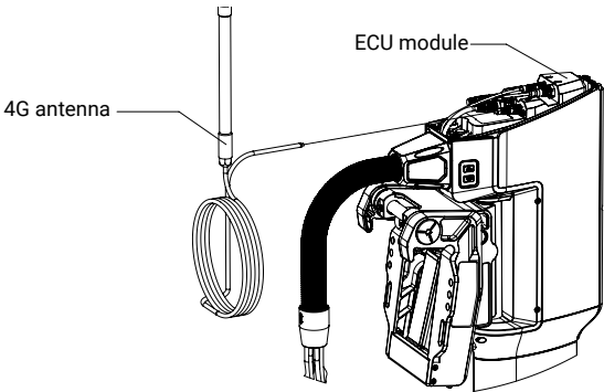
Figure 4.16 Connection between the 4G antenna and the outboard motor
