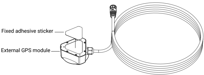
Figure 4.18 GPS external module adhesive pad fixing
