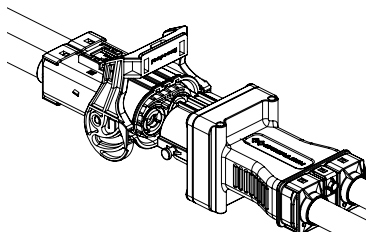
Figure 4.9 High-voltage interlock connector - Installation step 2
